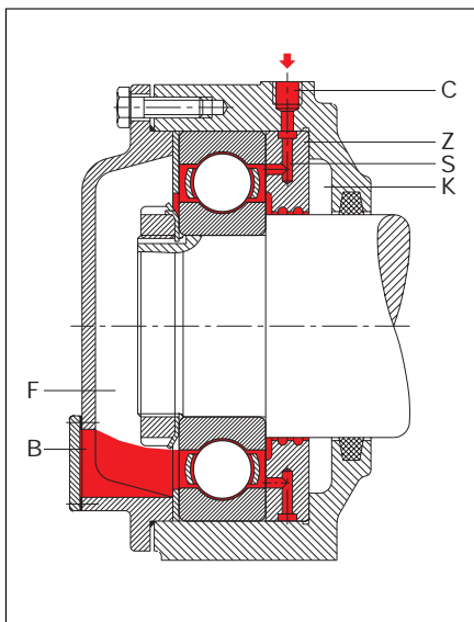
45: Direct supply of grease from the side through holes in a feed disk
